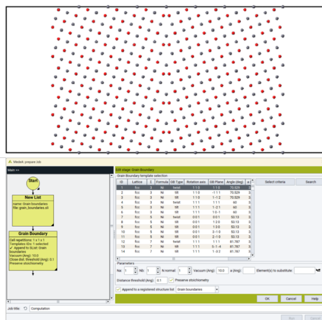
Create High-symmetry grain boundaries with the Interface Builder
